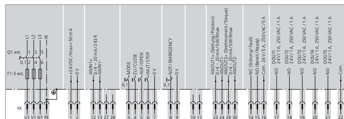
TPC terminal plan extract for AC controls
